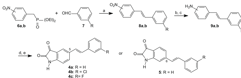
Scheme 1. Synthetic pathway to analogues 4a–c of ( E )-5-styrylisatin and ( E )-6-styrylisatin ( 5 ). Reagents and conditions: (a) NaOEt (b) \text{SnCl}_2/\text{HCl} , reflux (c) NaOH (d) diethyl ketomalonate, \text{CH}_3\text{CO}_2\text{H} , 120^\circ\text{C} (e) air, 120^\circ\text{C} .
