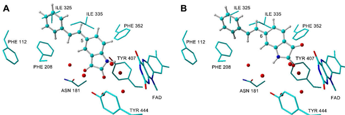
Figure 4. The docking solutions obtained with LigandFit for the binding of 4a (A) and 5 (B) in the active site of MAO-A (2Z5X.pdb). 14 The models were generated in Yasara. 18
