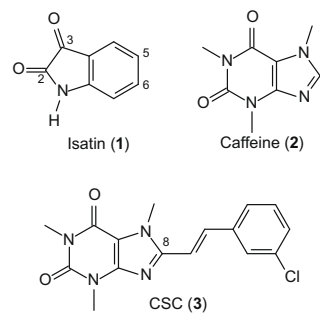
Figure 1. The structures of isatin ( 1 ), caffeine ( 2 ) and CSC ( 3 ).
