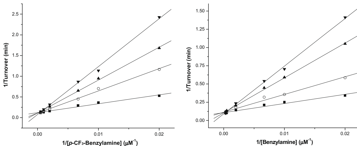
Figure 3. Lineweaver–Burk plots of the recombinant human MAO-A (left) and MAO-B (right). The activity of MAO-A (left) was assayed at varied concentrations of p -CF 3 -benzylamine with constant inhibitor concentrations of: (■) 0.0 μM of 4a , (○) 1.0 μM of 4a , (▲) 2.0 μM of 4a , (▼) 3.0 μM of 4a . The activity of MAO-B (right) was assayed at varied concentrations of benzylamine with constant inhibitor concentrations of: (■) 0.0 μM of 4a , (○) 0.3 μM of 4a , (▲) 0.7 μM of 4a , (▼) 1.0 μM of 4a .
